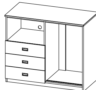
Entertainment Unit 47.75 X 23.75 X 40.5
