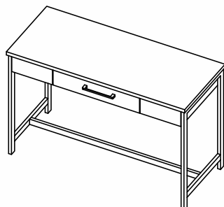
Desk w/ Drawer 47.75 X 23.75 X 31
